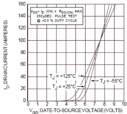
FIGURE 4, TRANSFER CHARACTERISTICS
